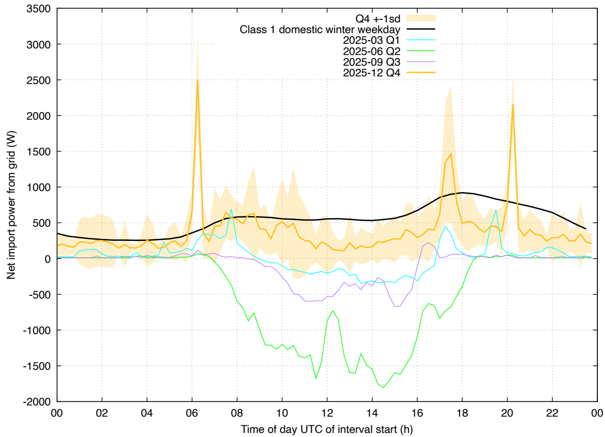
16WW Grid Net Load Profiles (weekday) 2025
