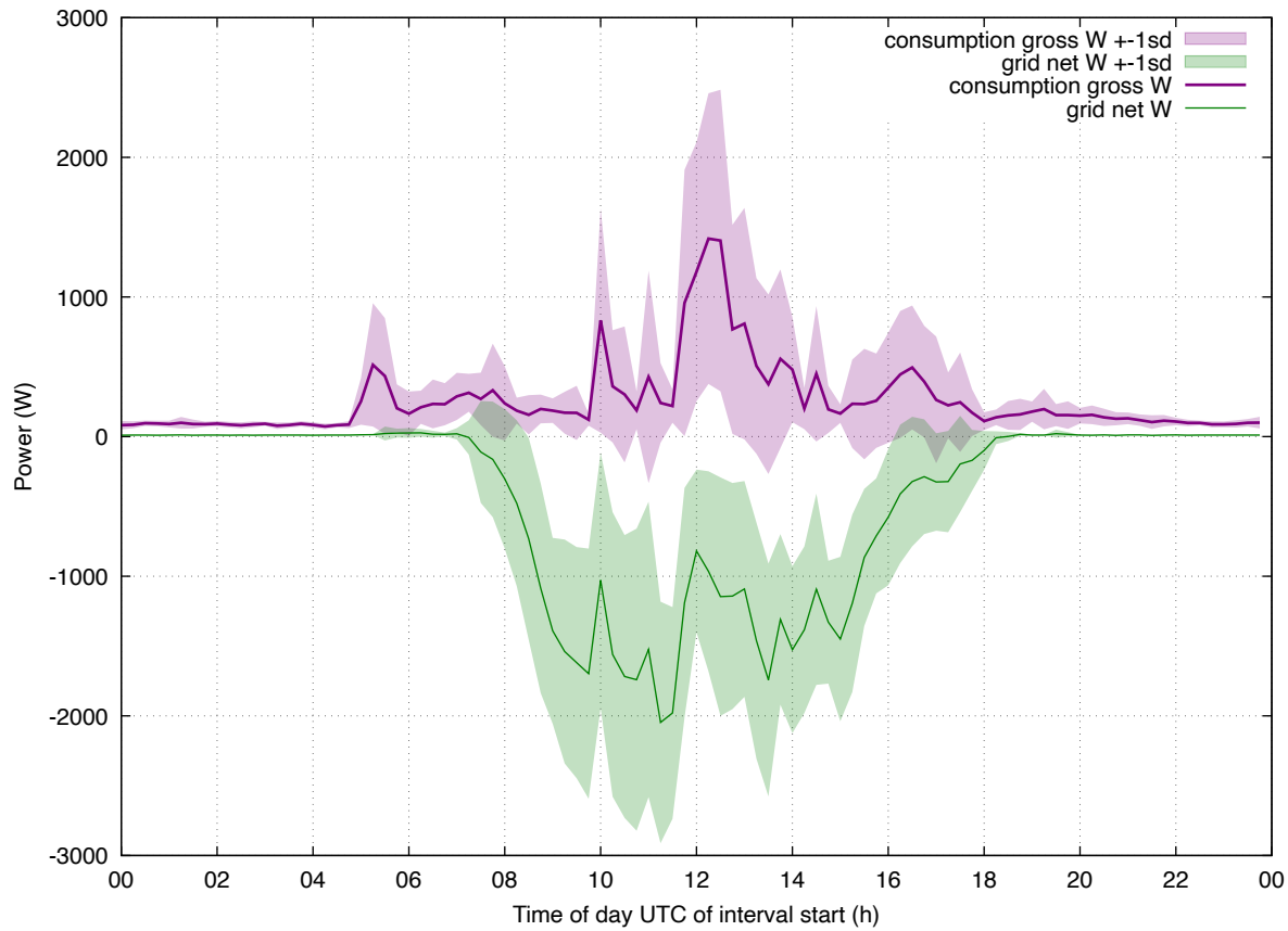
Load Profile: 202608 enphase weekend
