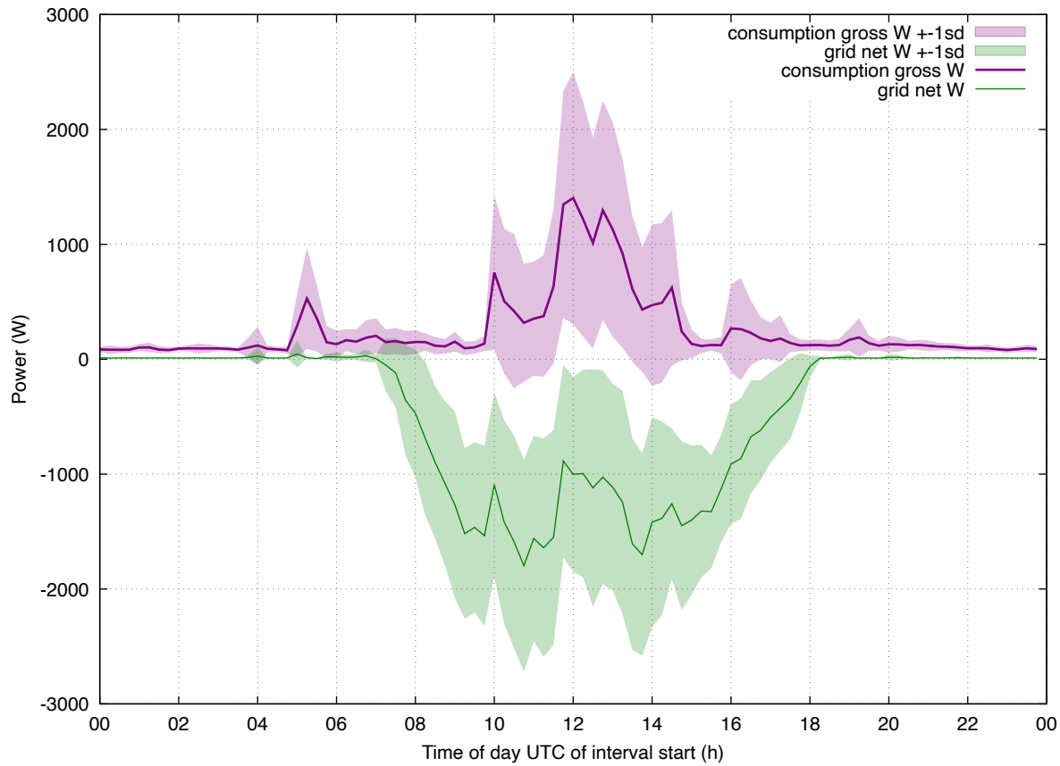
Load Profile: 202608 enphase weekday
