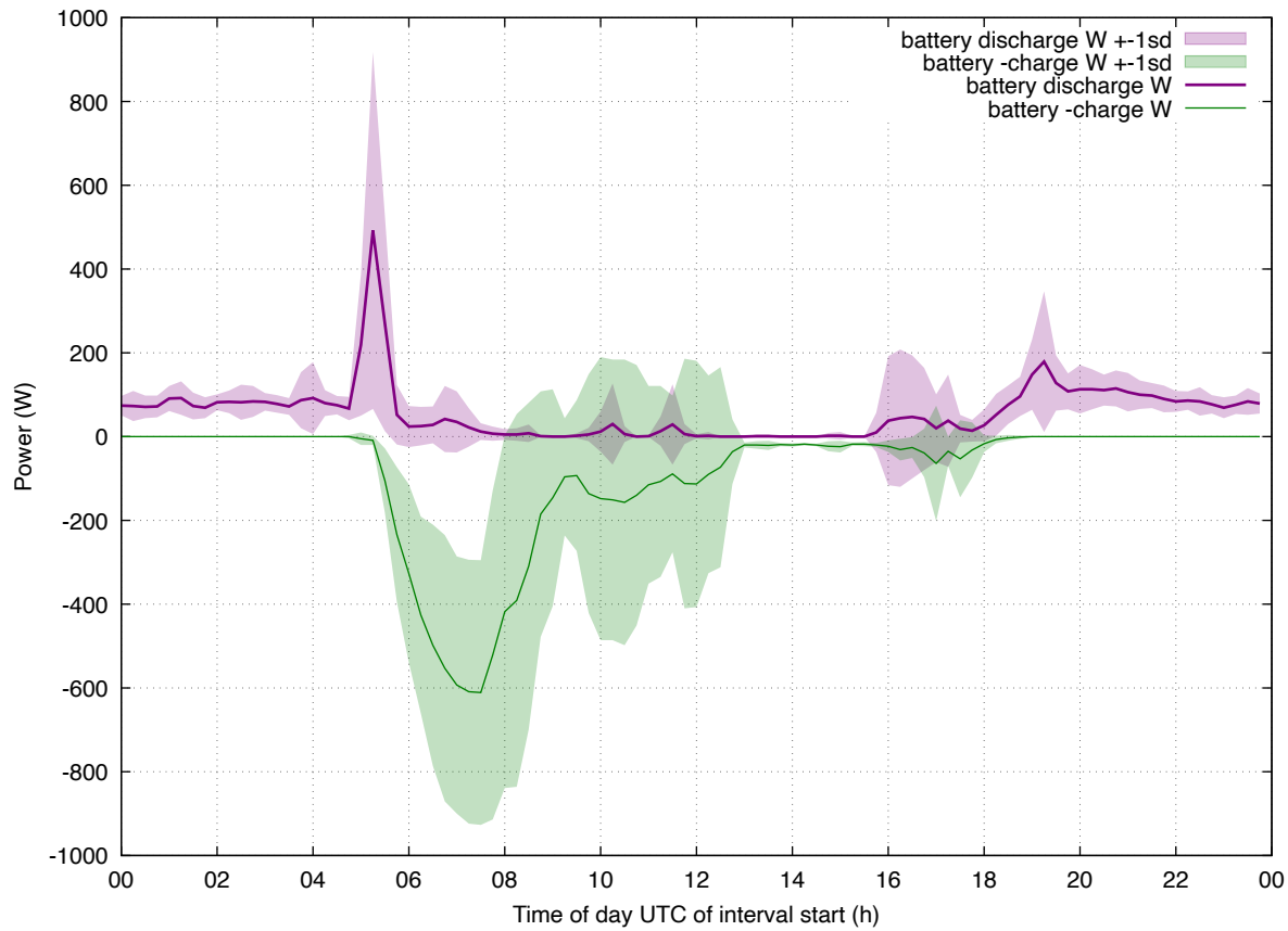
Load Profile: 202608 enphase-batt weekday
