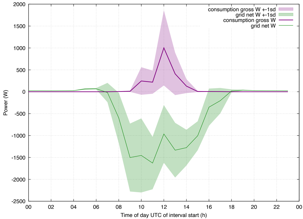
Load Profile: 202608 eddi-iheat weekend
