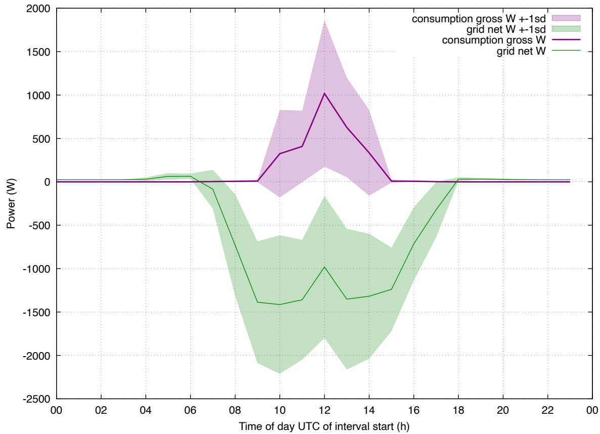
Load Profile: 202608 eddi-iheat weekday
