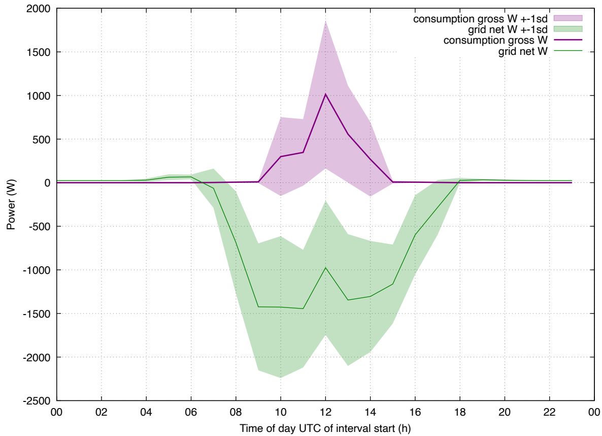
Load Profile: 202608 eddi-iheat all
