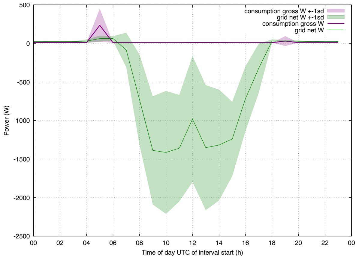
Load Profile: 202608 eddi-hph4 weekday
