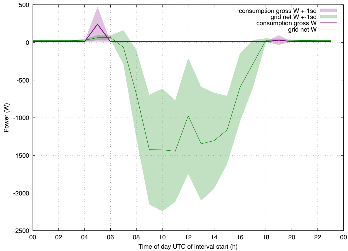
Load Profile: 202608 eddi-hph4 all
