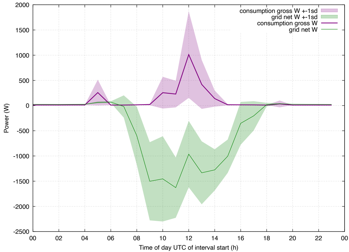
Load Profile: 202608 eddi-eheat weekend
