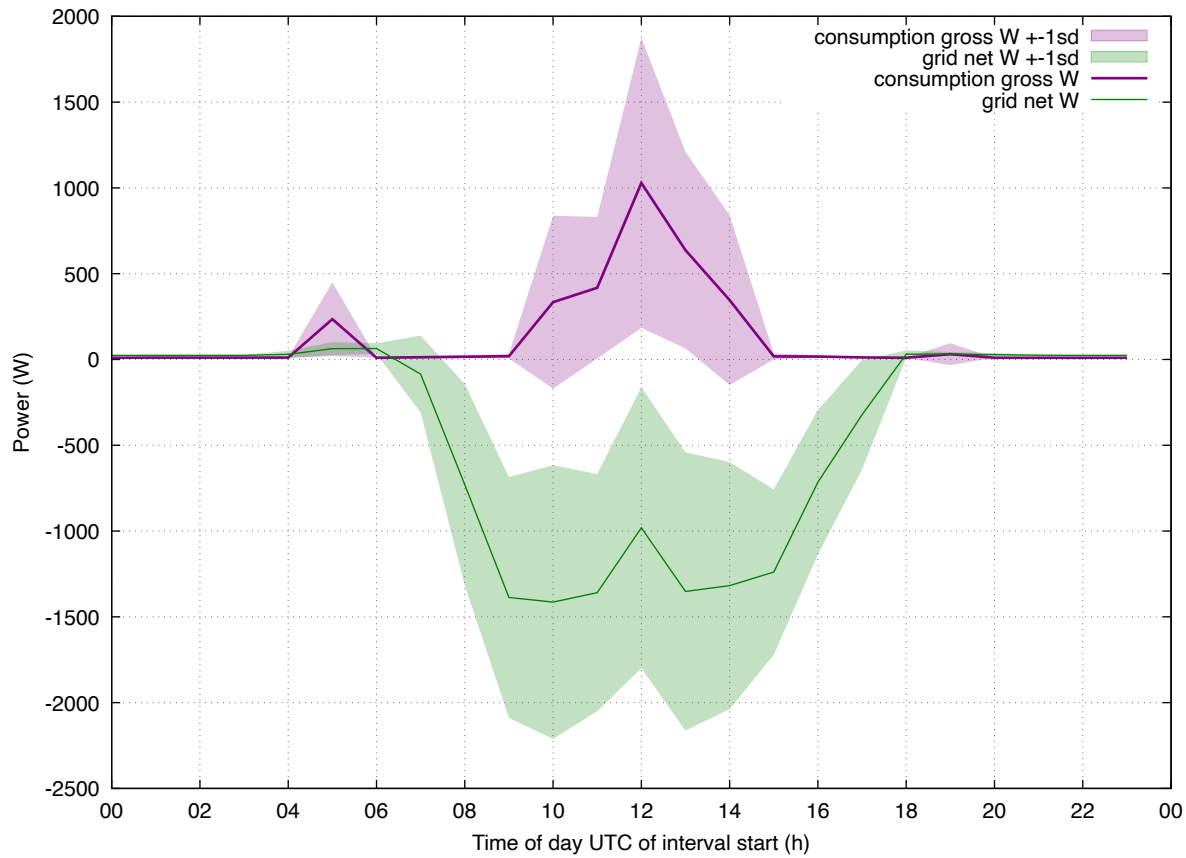
Load Profile: 202608 eddi-eheat weekday
