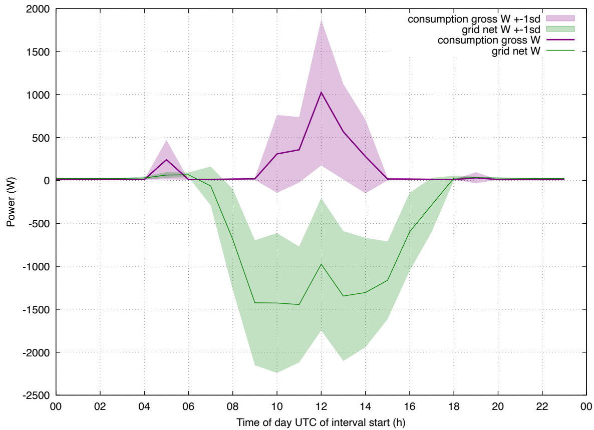
Load Profile: 202608 eddi-eheat all
