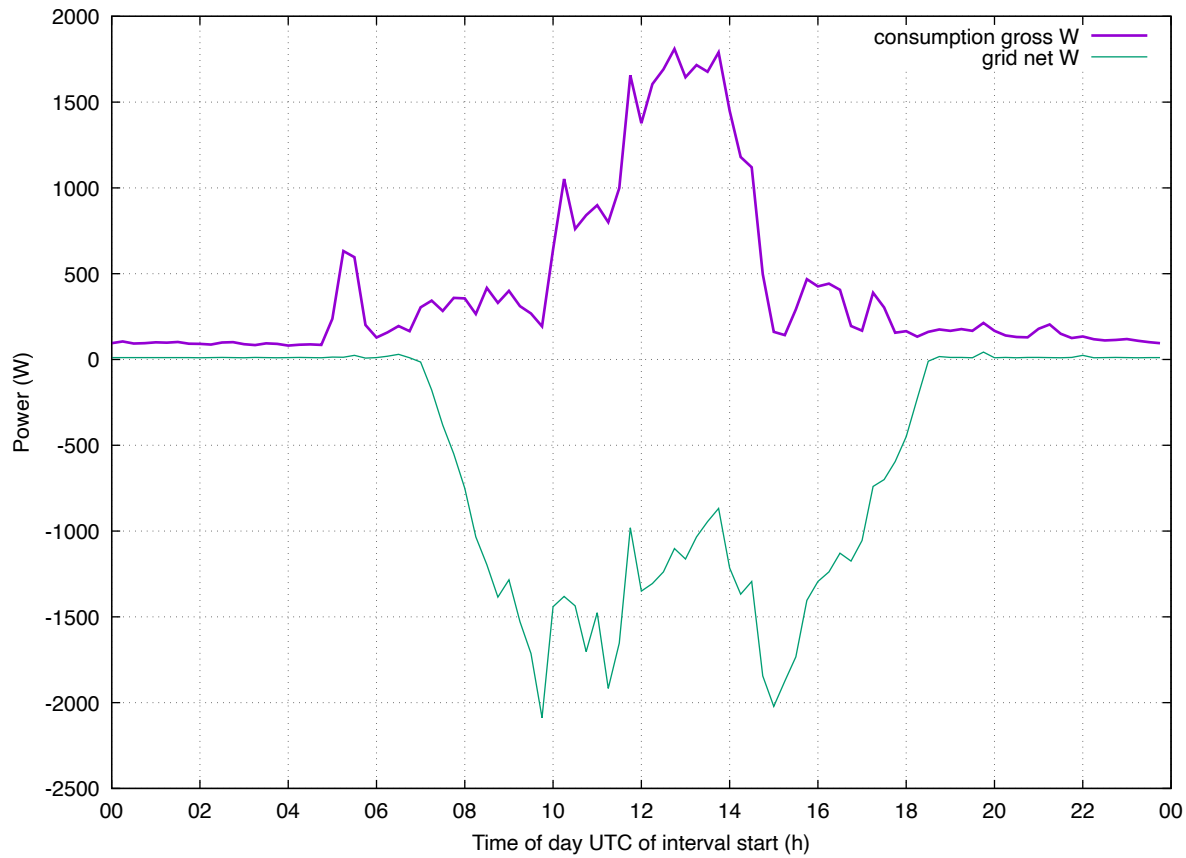
Load Profile: 202607 enphase weekend
