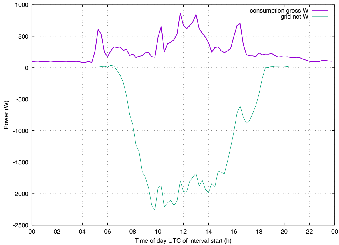
Load Profile: 202607 enphase weekday
