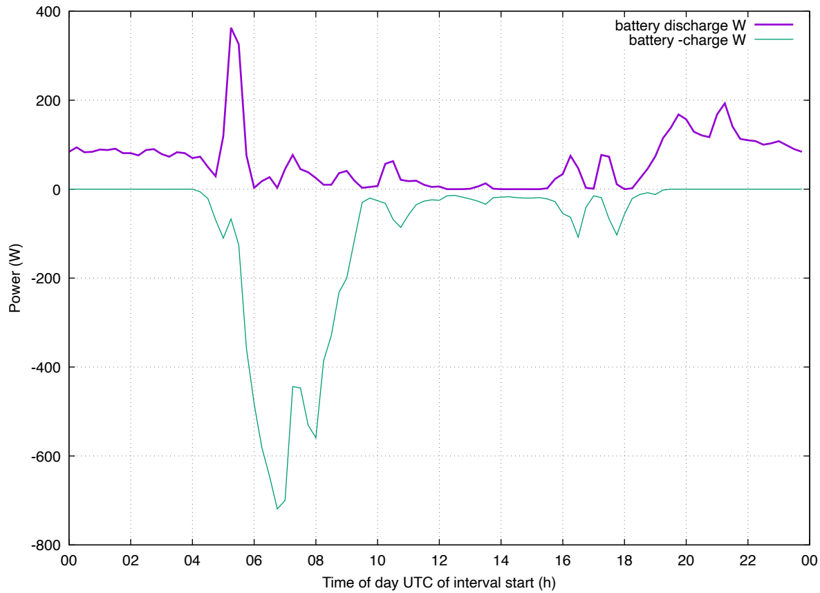
Load Profile: 202607 enphase-batt weekend
