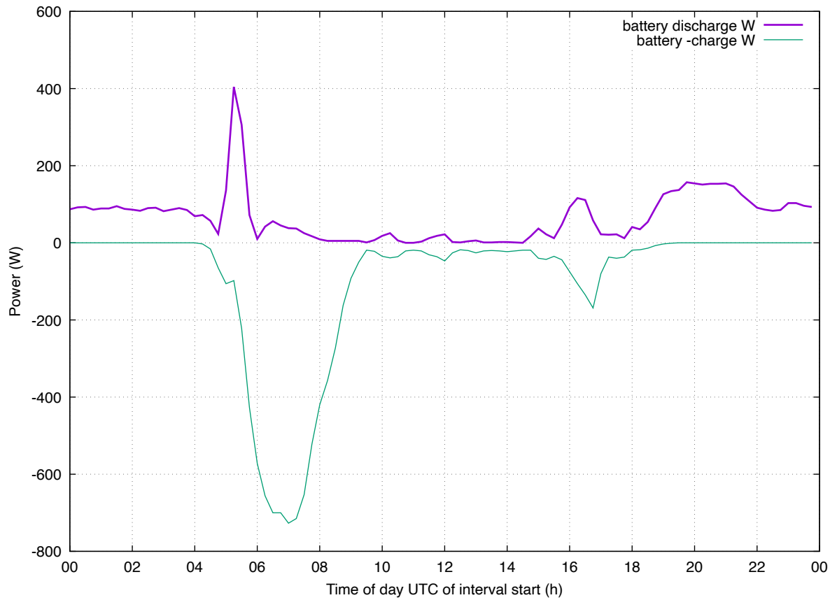
Load Profile: 202607 enphase-batt weekday
