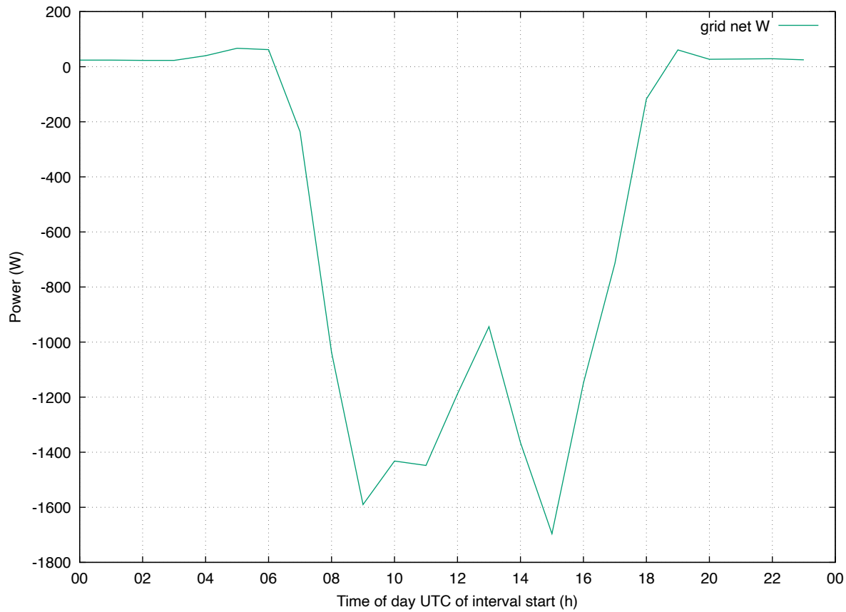
Load Profile: 202607 eddi weekend
