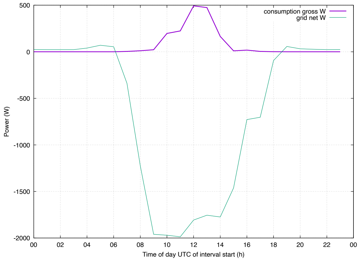
Load Profile: 202607 eddi-iheat weekday
