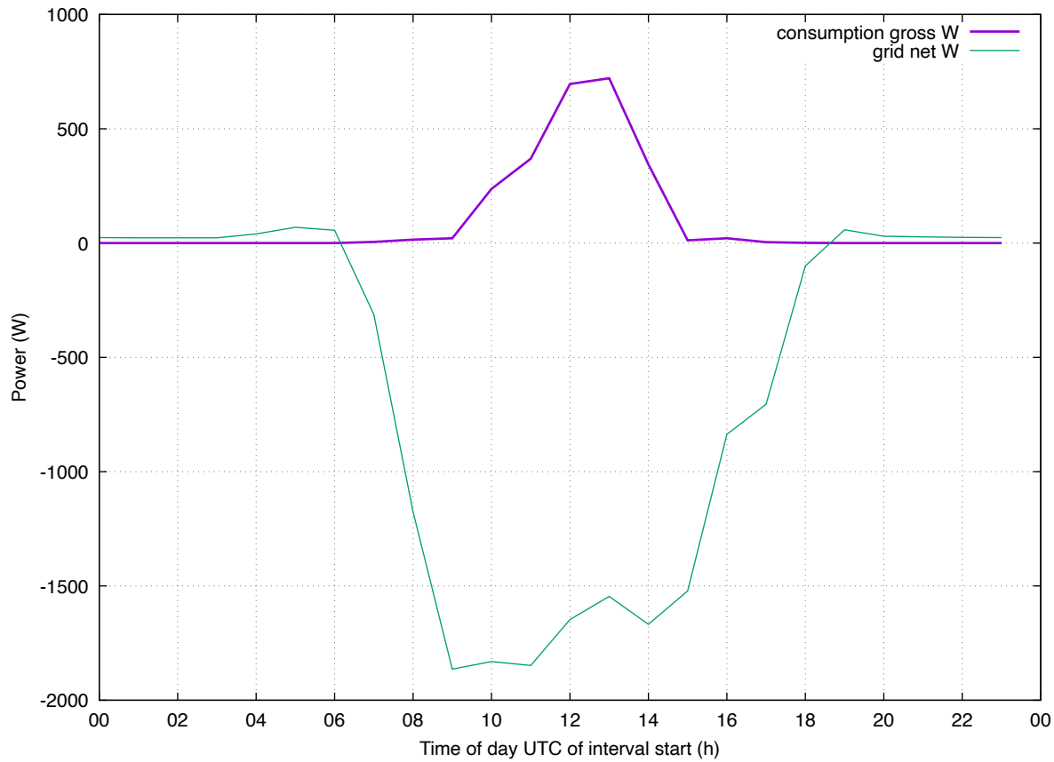
Load Profile: 202607 eddi-iheat all
