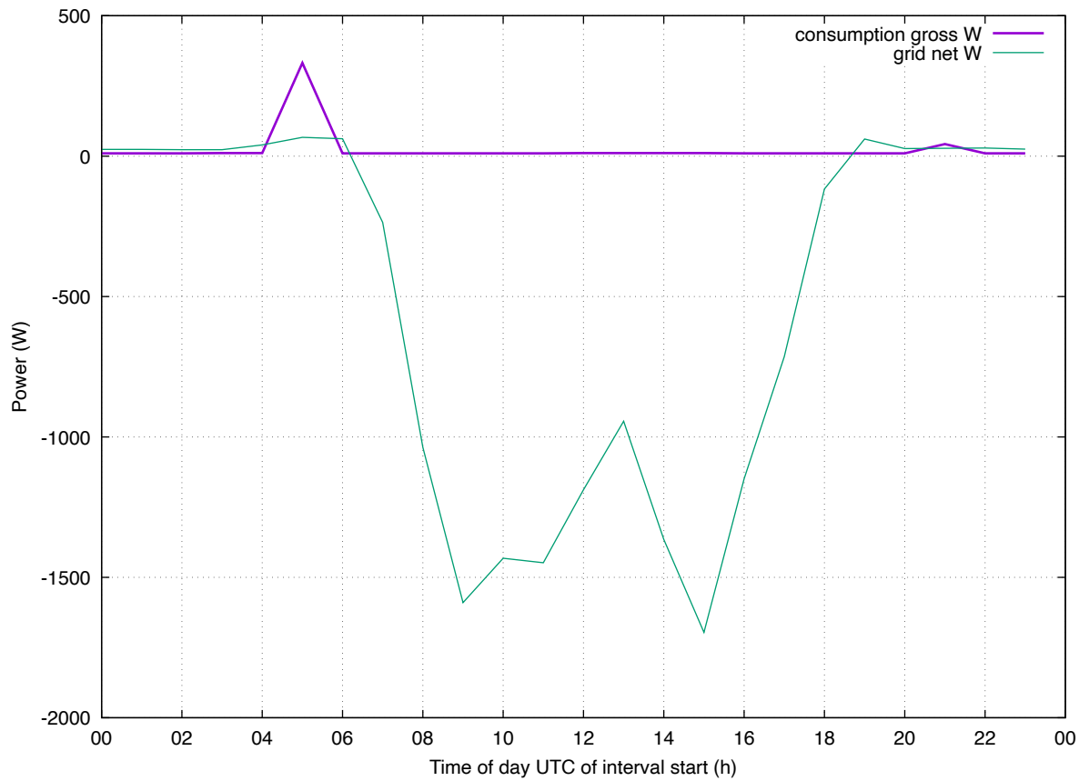
Load Profile: 202607 eddi-hph4 weekend
