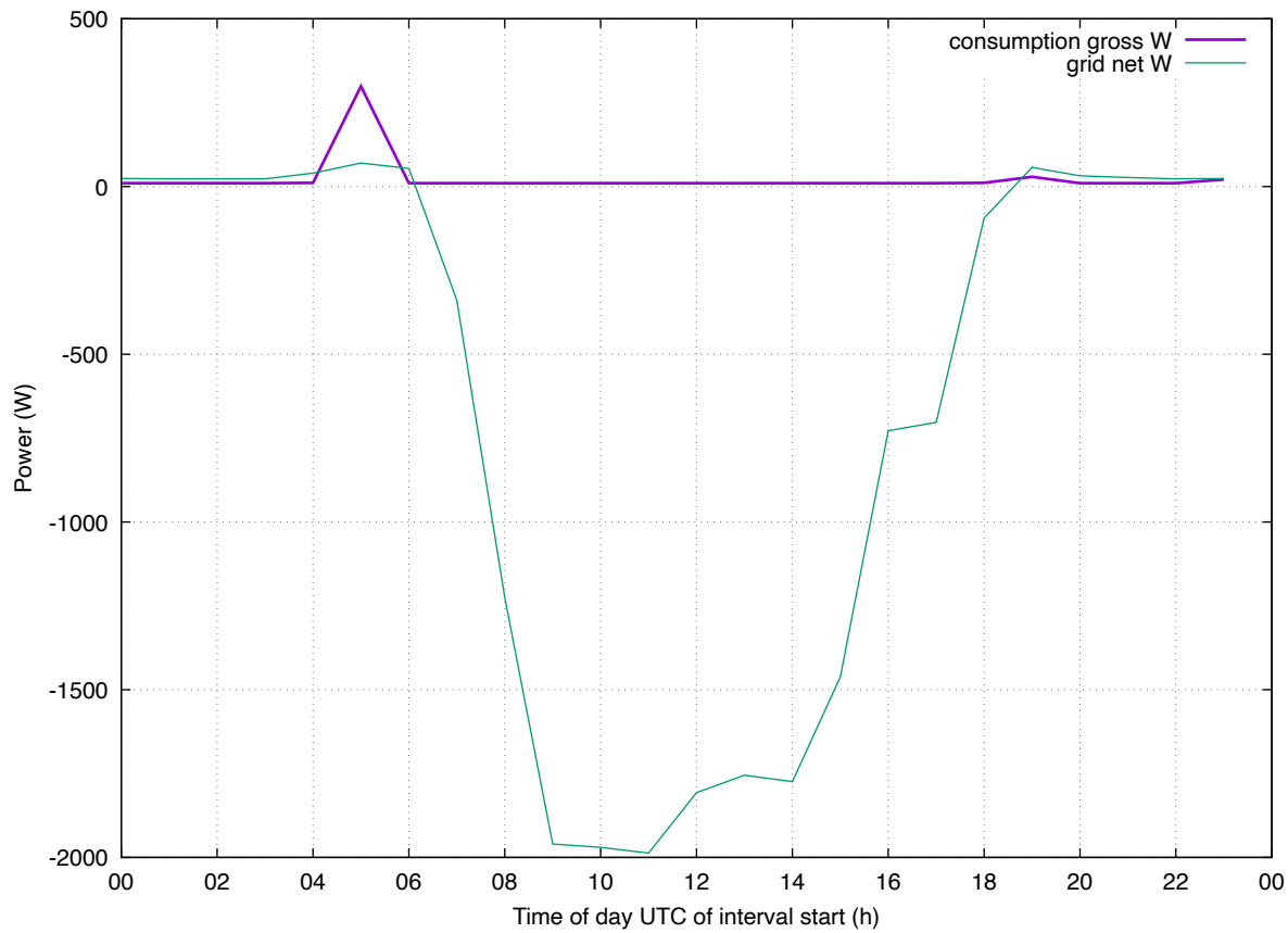
Load Profile: 202607 eddi-hph4 weekday
