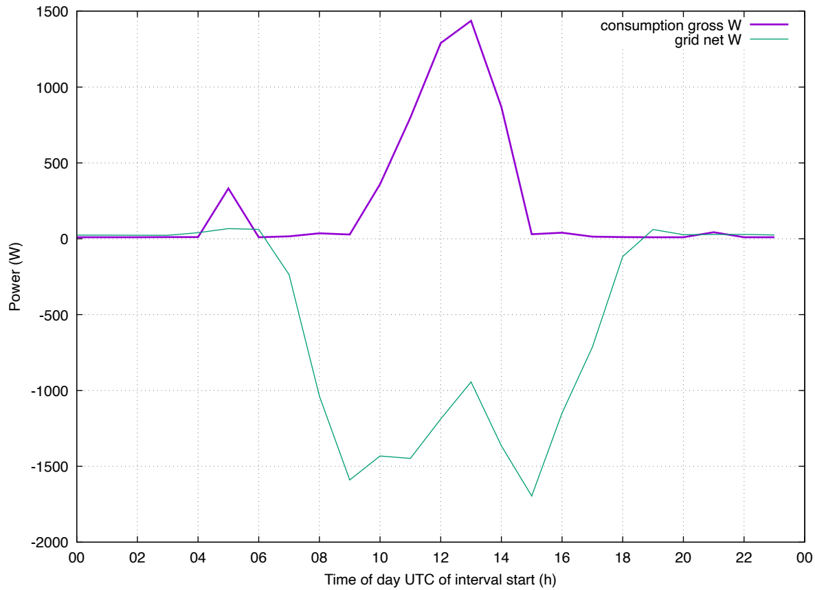
Load Profile: 202607 eddi-ehat weekend
