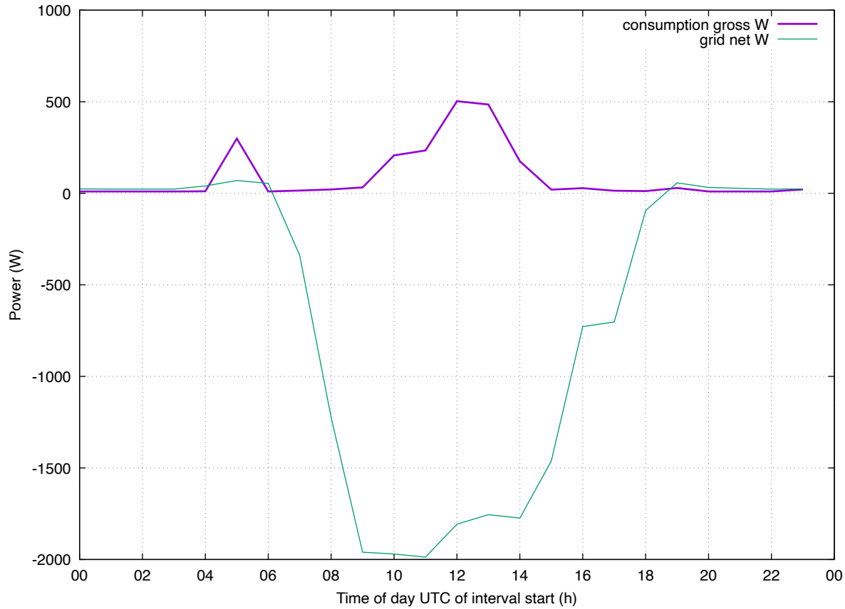
Load Profile: 202607 eddi-eheat weekday
