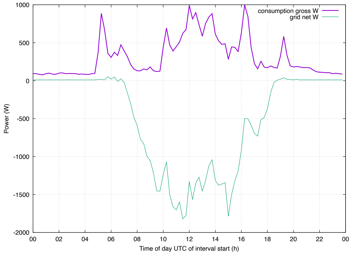
Load Profile: 202606 enphase weekday
