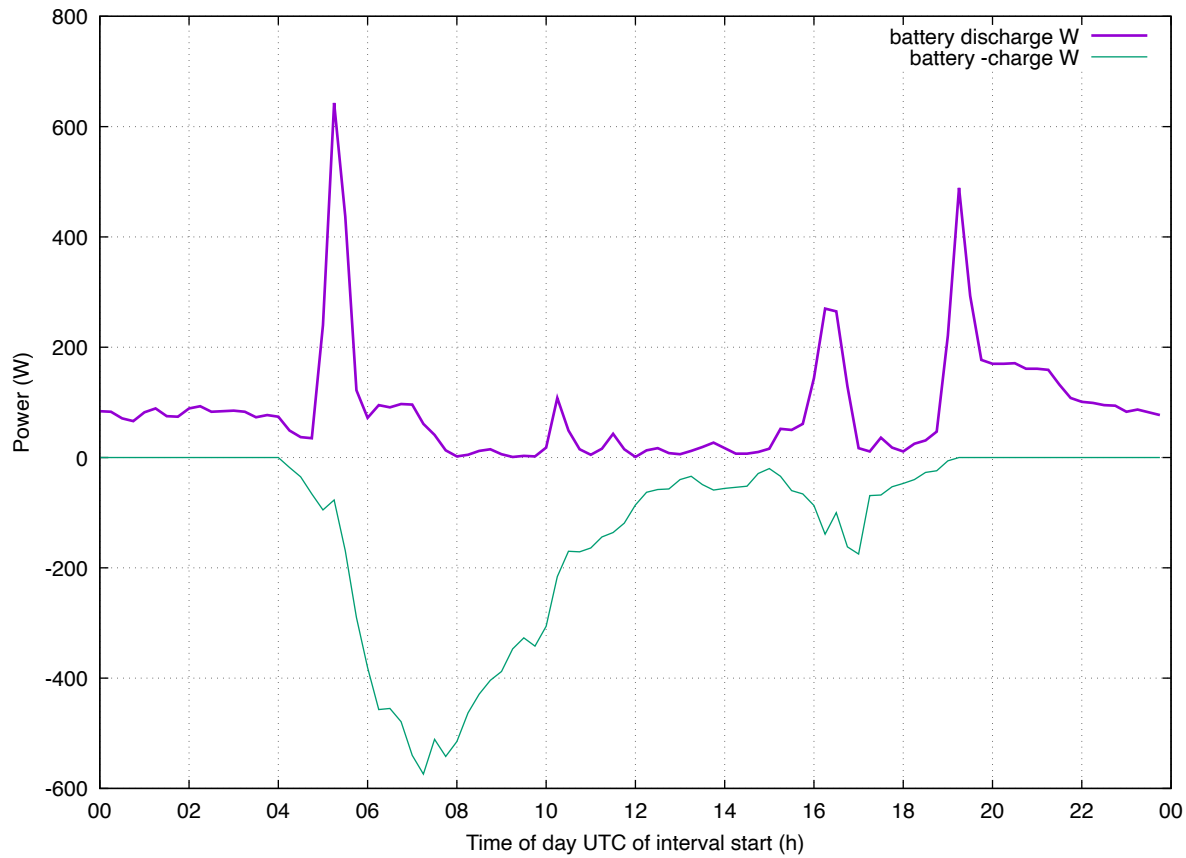
Load Profile: 202606 enphase-batt weekday
