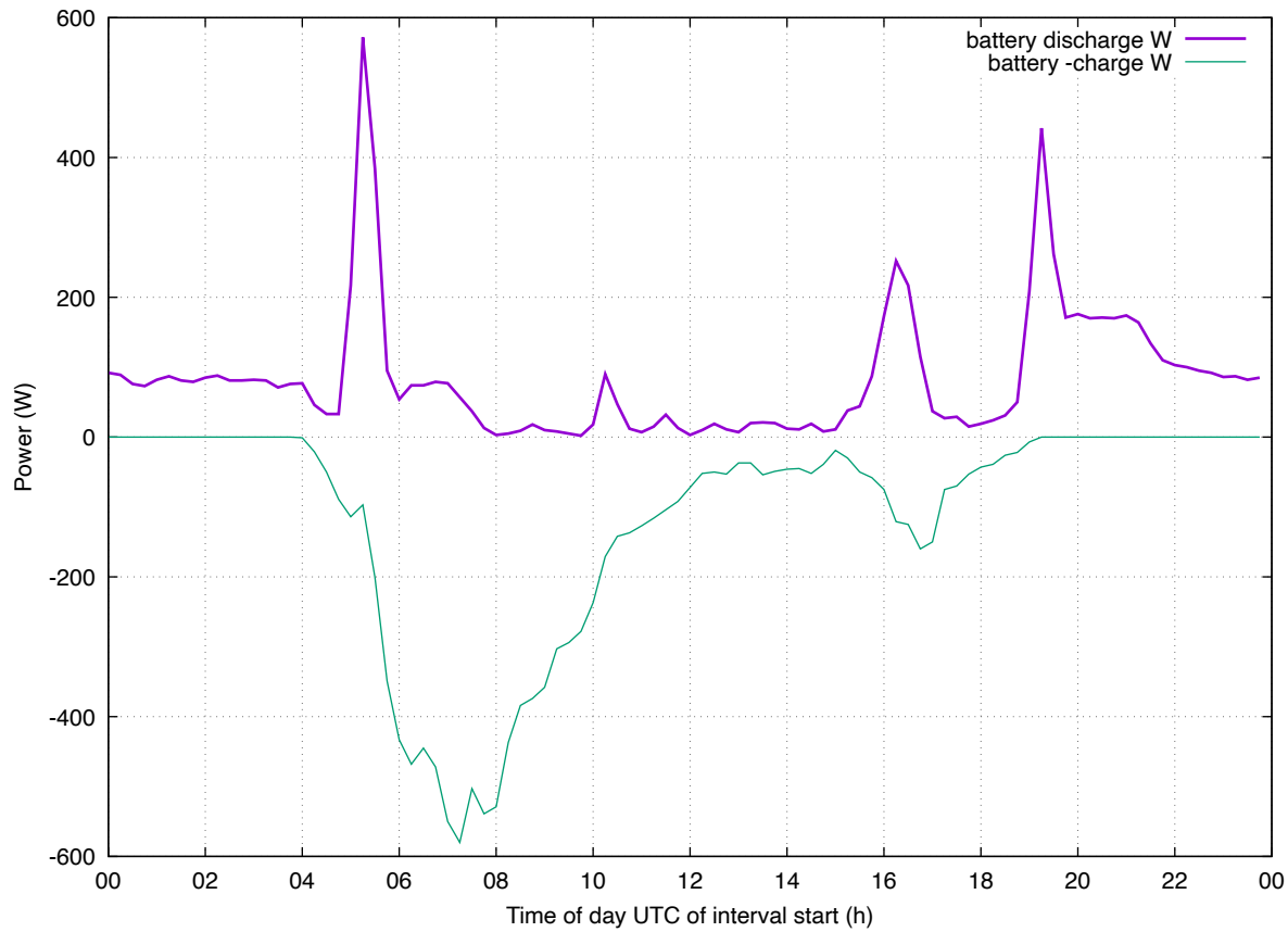
Load Profile: 202606 enphase-batt all
