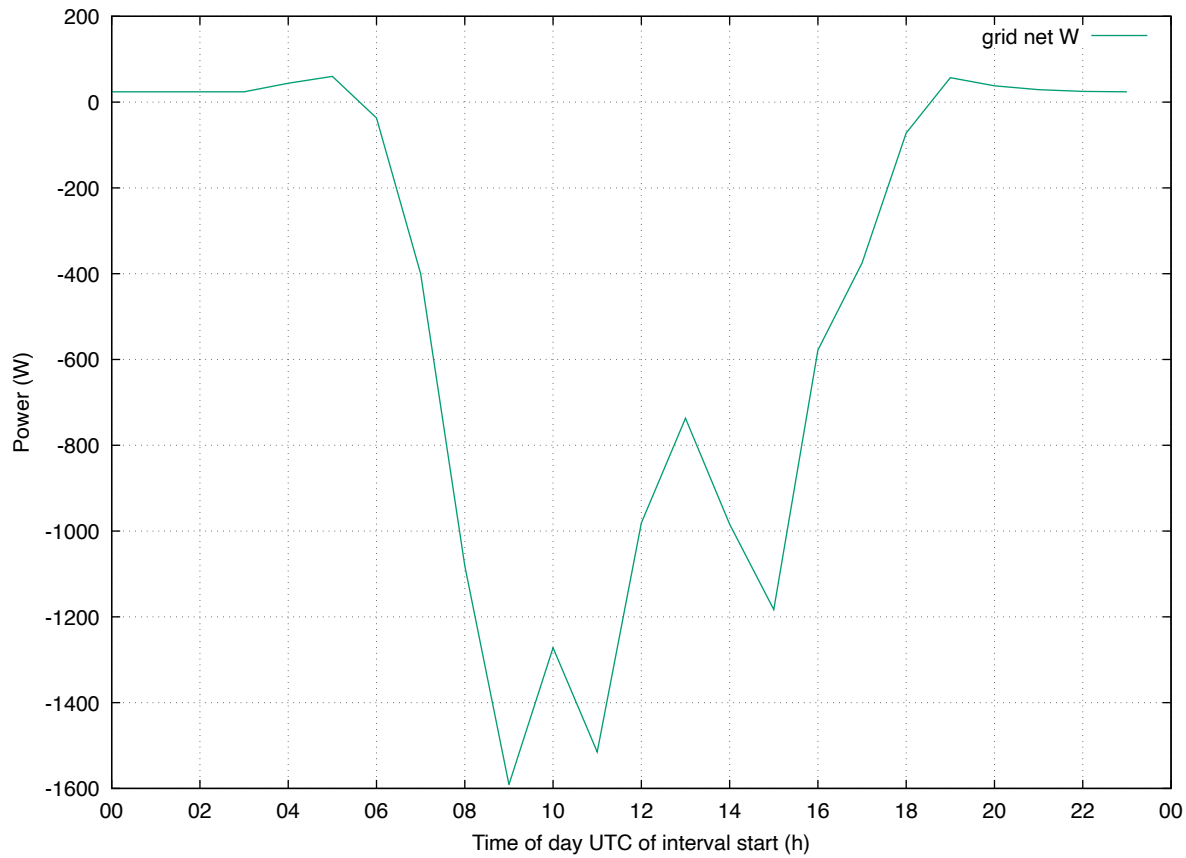
Load Profile: 202606 eddi weekend
