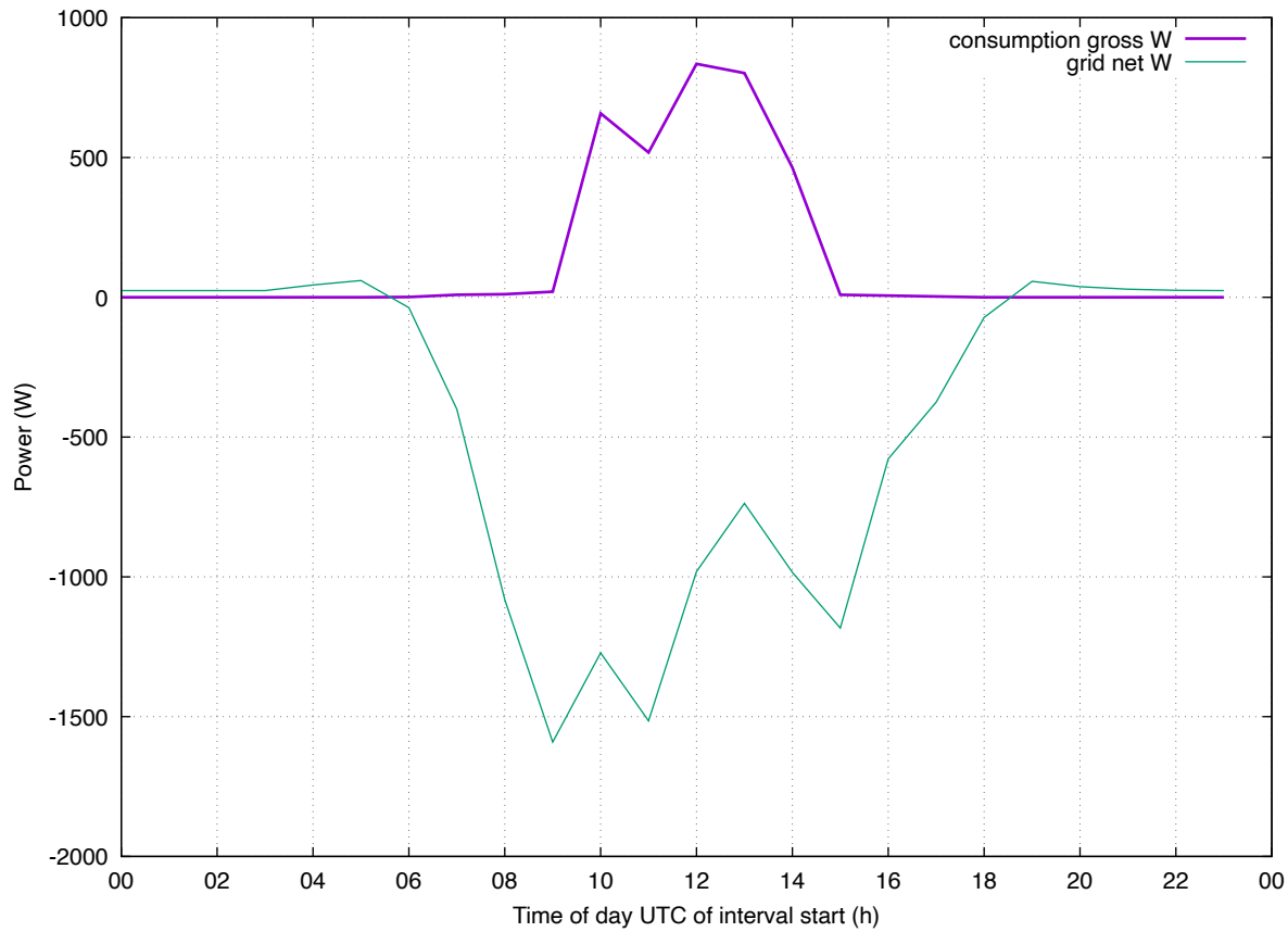
Load Profile: 202606 eddi-iheat weekend
