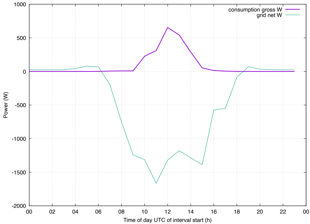
Load Profile: 202606 eddi-heat weekday
