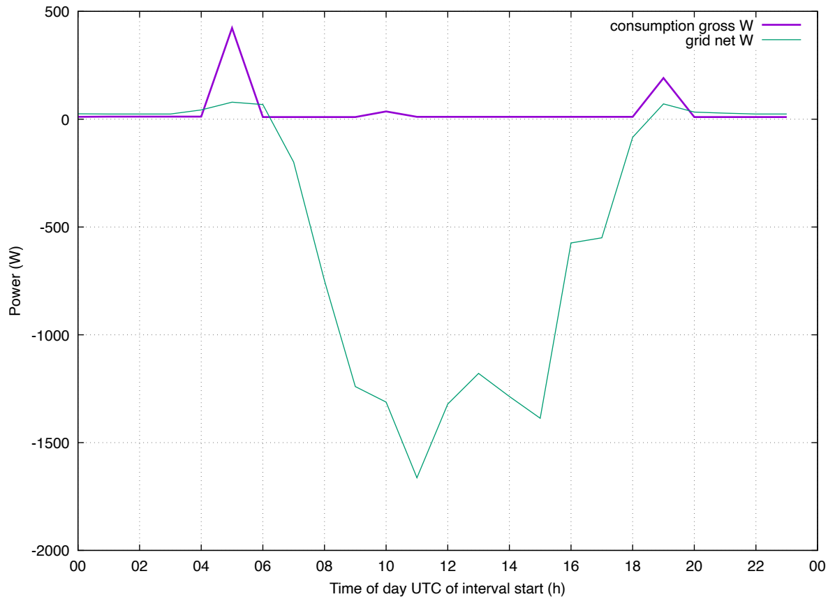
Load Profile: 202606 eddi-hph4 weekday
