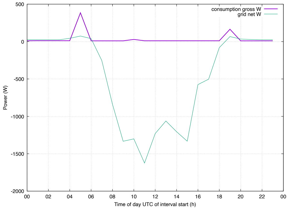
Load Profile: 202606 eddi-hph4 all
