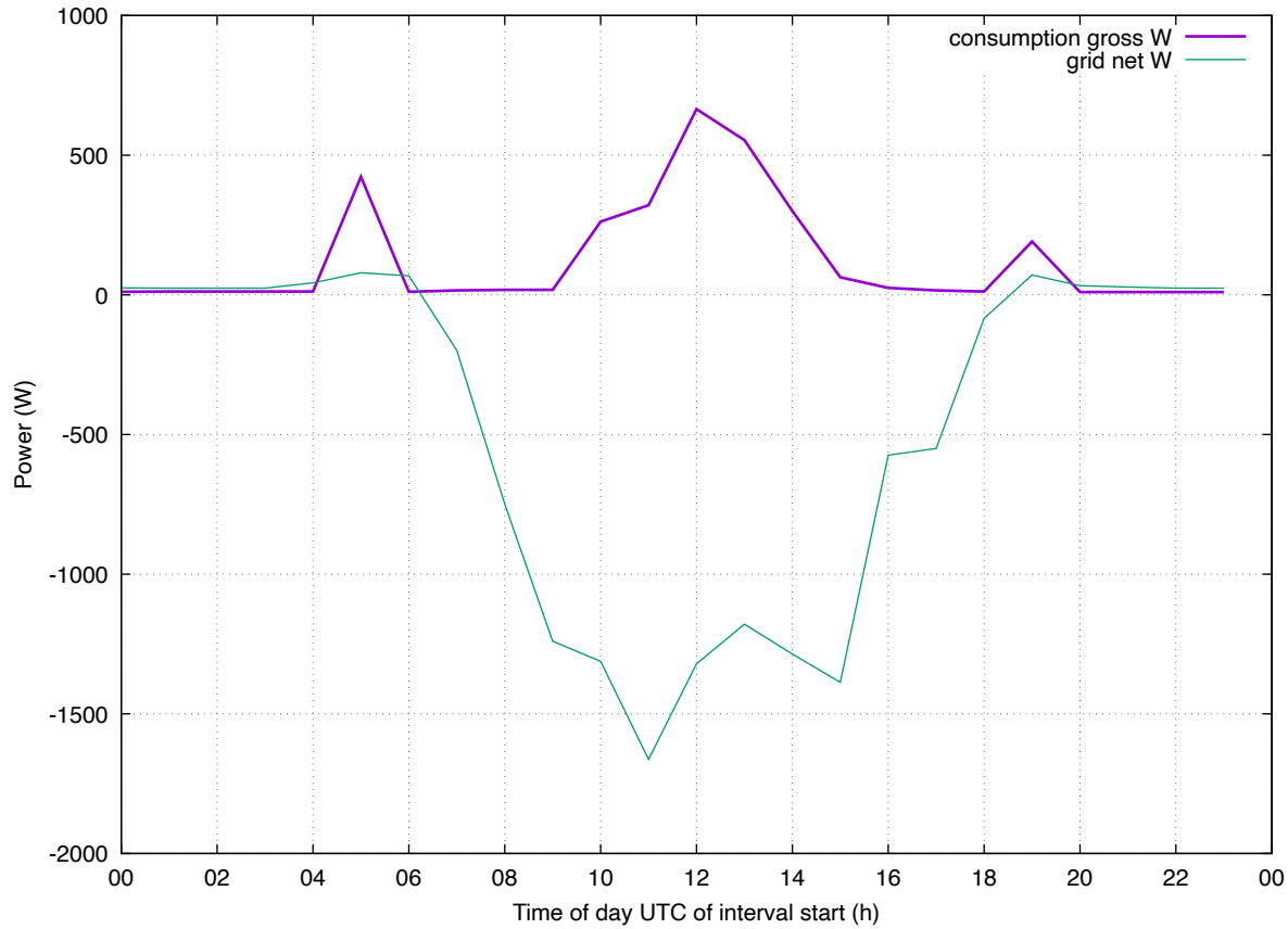
Load Profile: 202606 eddi-eheat weekday
