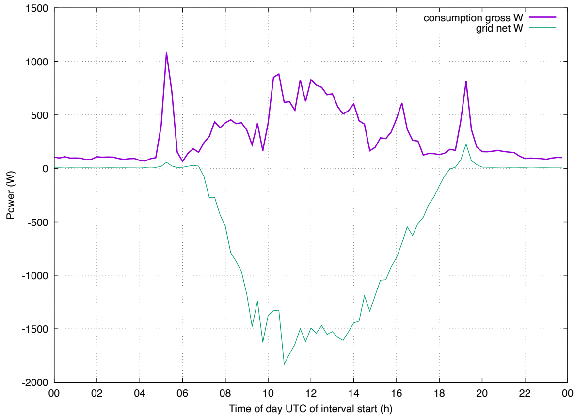
Load Profile: 202605 enphase weekend
