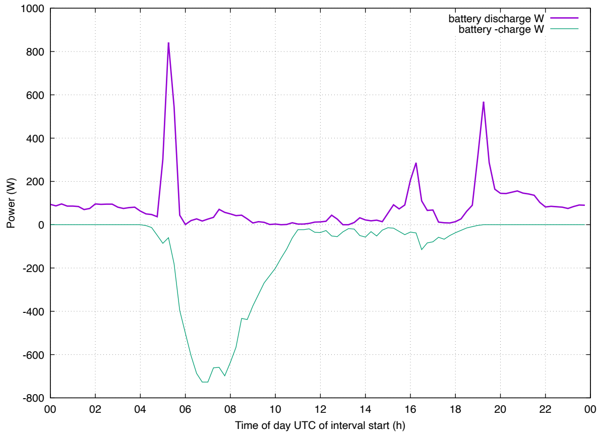
Load Profile: 202605 enphase-batt weekend
