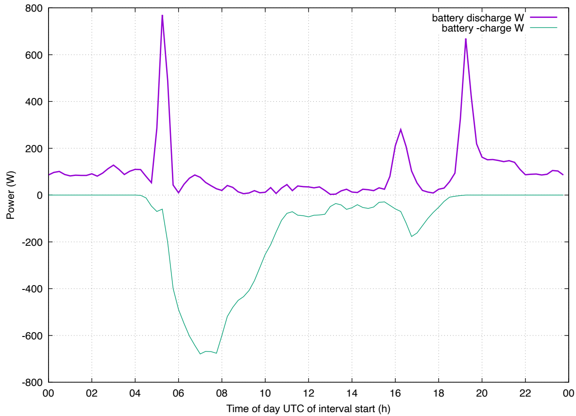
Load Profile: 202605 enphase-batt all
