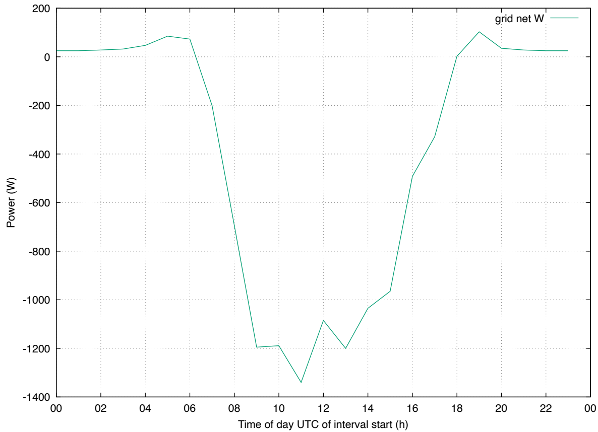
Load Profile: 202605 eddi all
