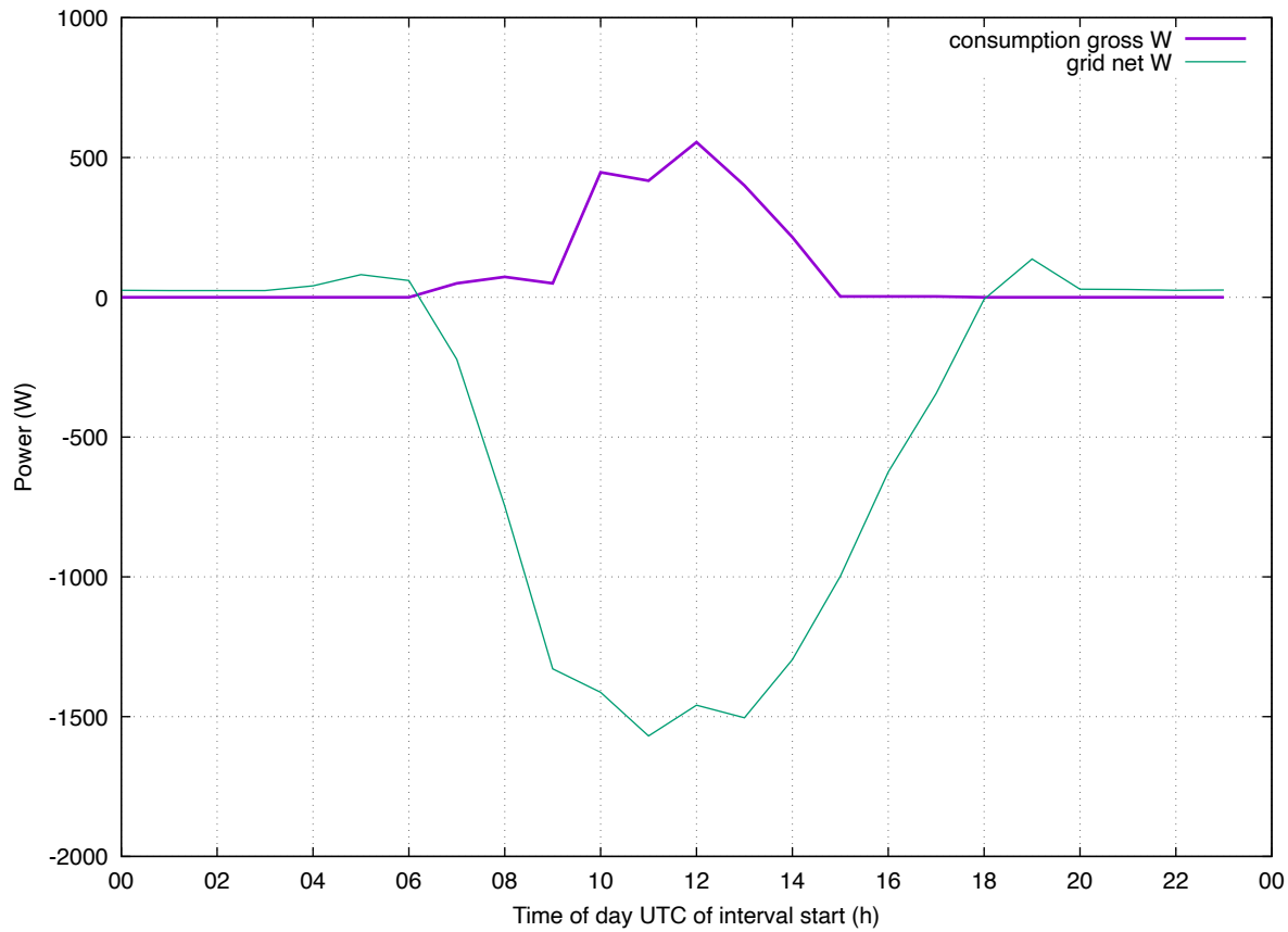
Load Profile: 202605 eddi-iheat weekend
