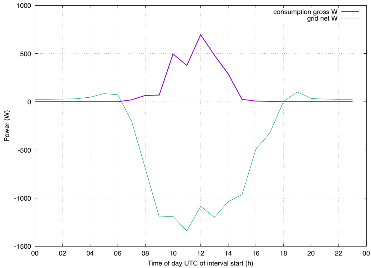
Load Profile: 202605 eddi-iheat all
