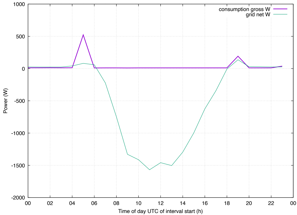
Load Profile: 202605 eddi-hph4 weekend
