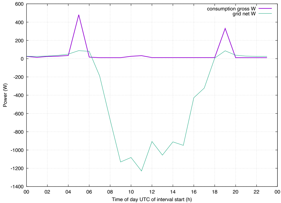
Load Profile: 202605 eddi-hph4 weekday
