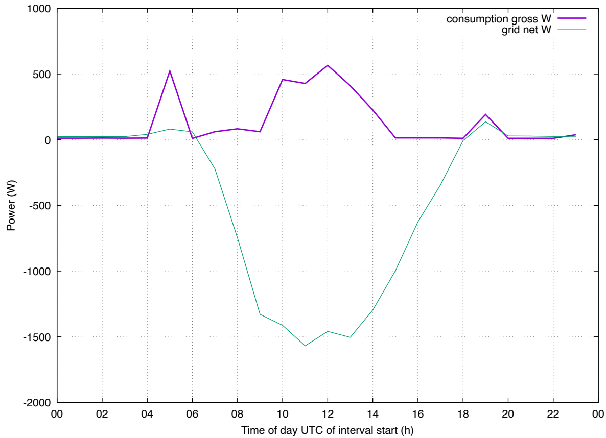
Load Profile: 202605 eddi-eheat weekend
