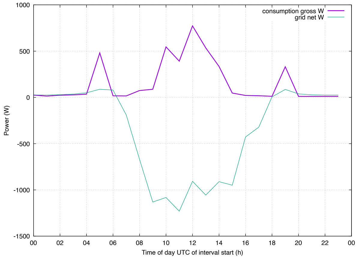
Load Profile: 202605 eddi-eheat weekday
