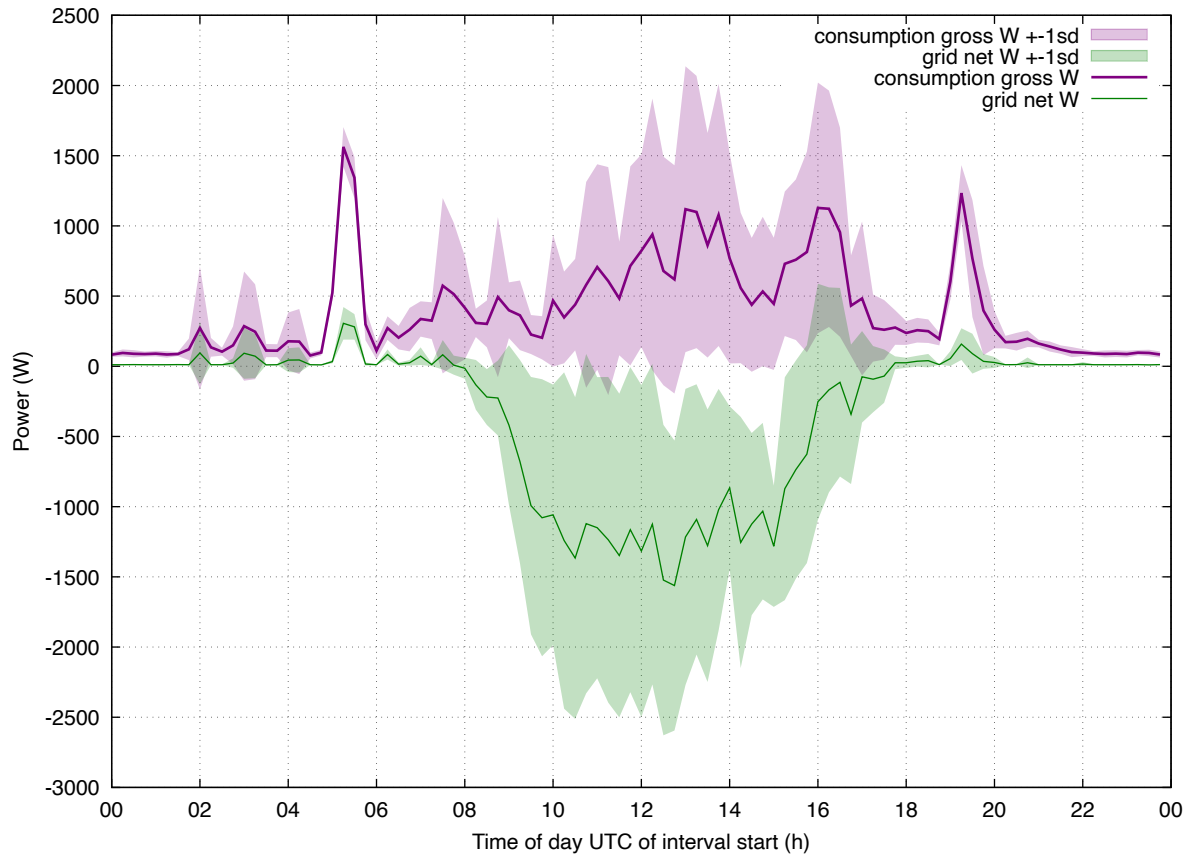
Load Profile: 202604 enphase weekend
