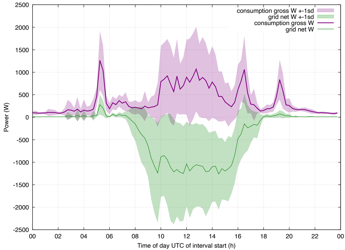
Load Profile: 202604 enphase weekday
