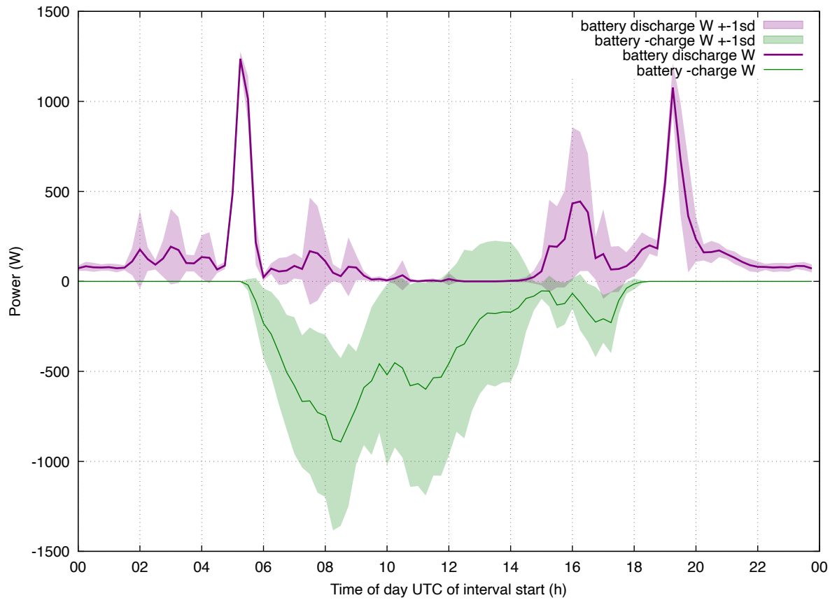
Load Profile: 202604 enphase-batt weekend
