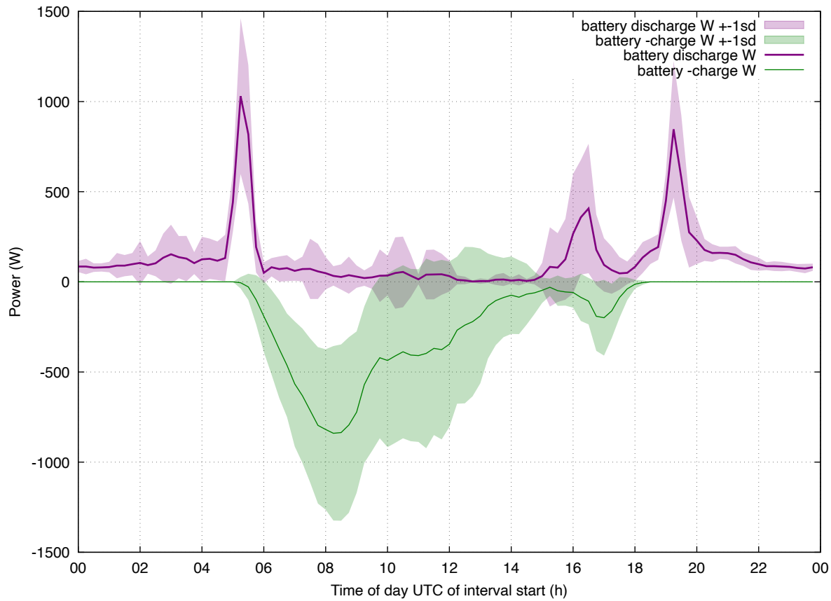
Load Profile: 202604 enphase-batt all
