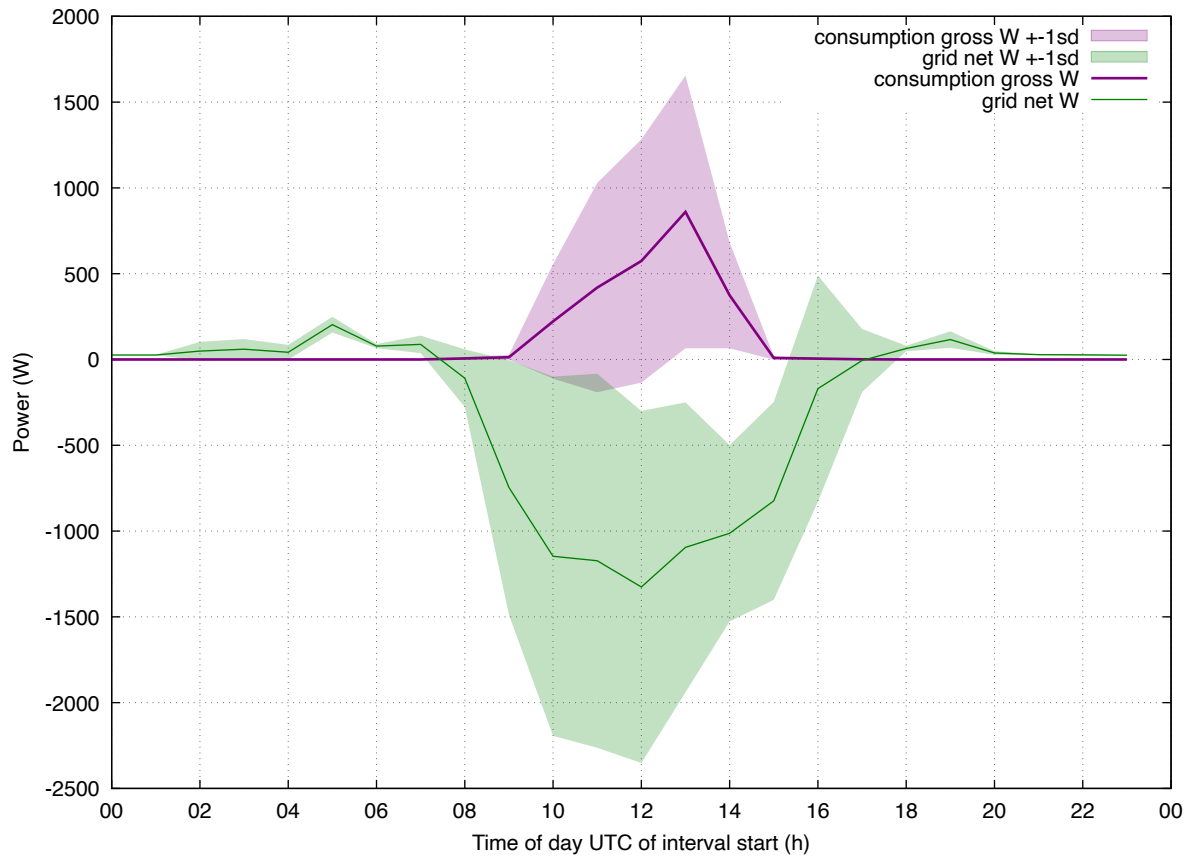
Load Profile: 202604 eddi-heat weekend
