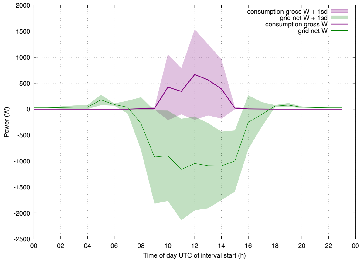
Load Profile: 202604 eddi-iheat weekday
