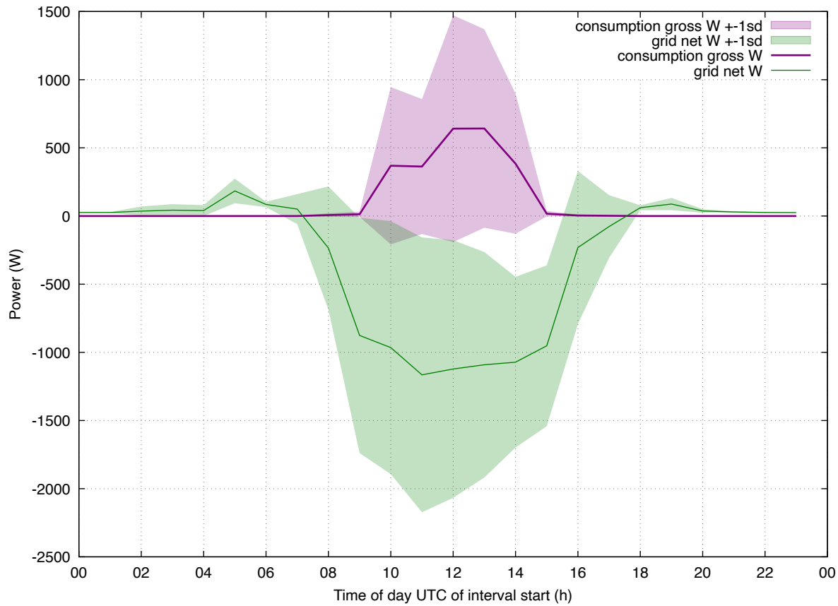
Load Profile: 202604 eddi-iheat all
