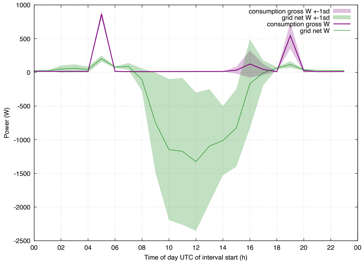
Load Profile: 202604 eddi-hph4 weekend
